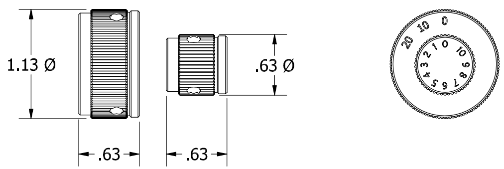
KNOB DETAIL
