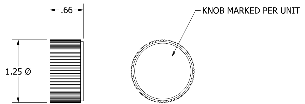
KNOB DETAIL
