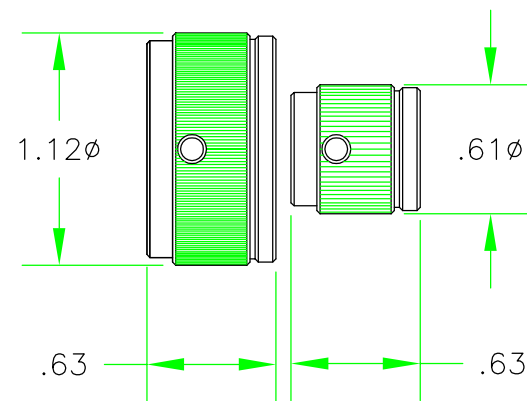
KNOB DETAIL
