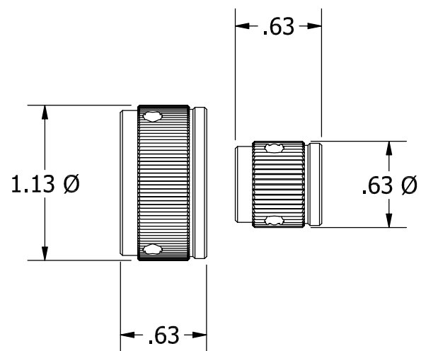
Knob Detail
