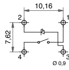
Single LED
